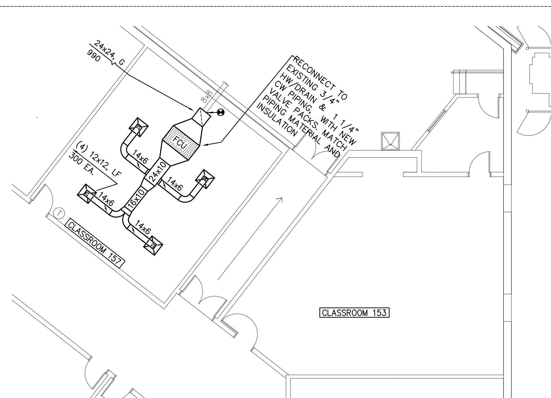
FIRST FLOOR PLAN CAD LAB - HVAC - NEW WORK SCALE : 1/8" = 1'-0"
