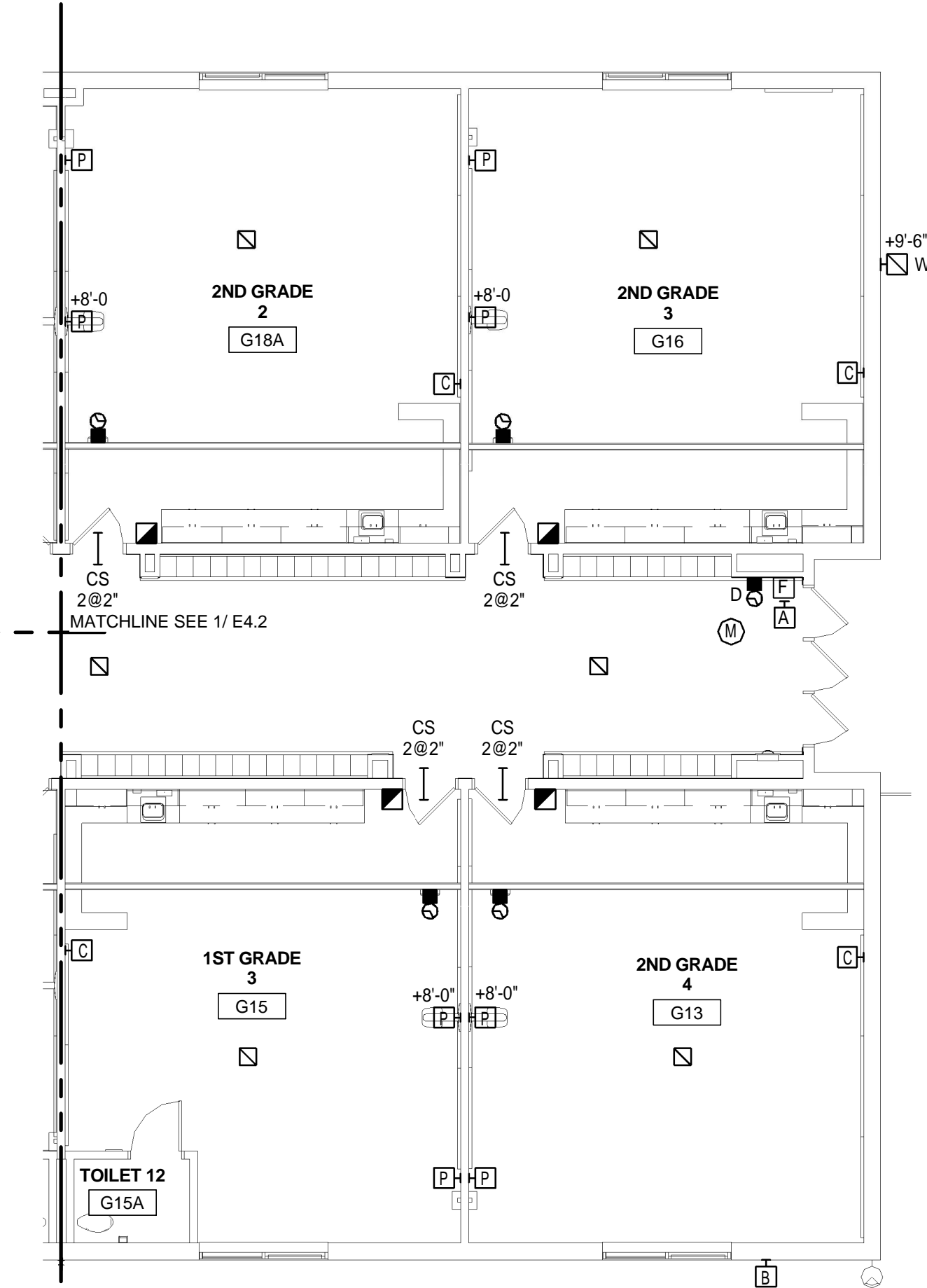
2 LEVEL 1 - ELECTRICAL LOW VOLTAGE PLAN - AREA C2 1/8" = 1'-0"
