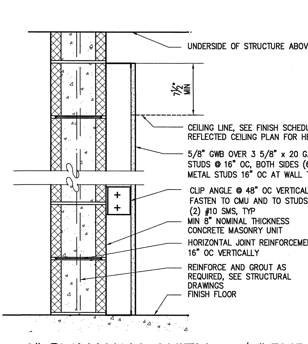
G 8" CMU WALL WITH 3 5/8" FURRING SCALE: 1 1/2"=1'-0" G6 8" CMU WALL WITH 6" FURRING SCALE: 1 1/2"=1'-0"
