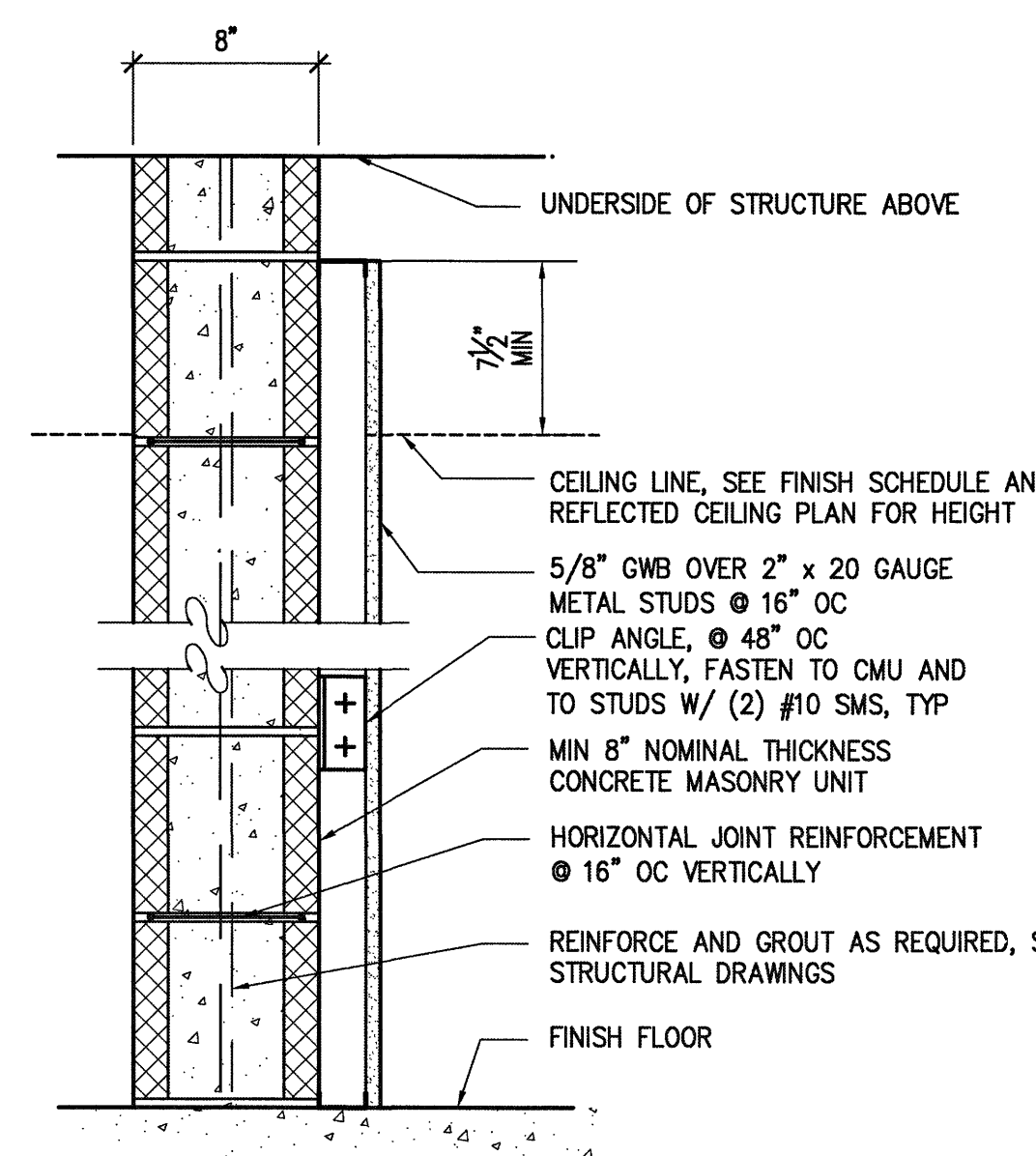
F 8" CMU WALL WITH 2" FURRING SCALE: 1 1/2"=1'-0"
