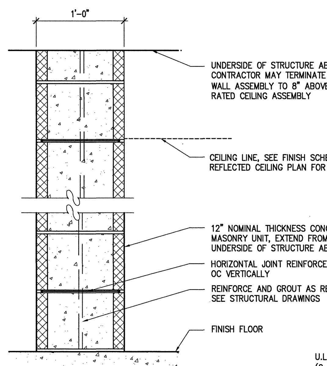
H ONE HOUR RATED 12" CMU WALL SCALE: 1 1/2"=1'-0"
