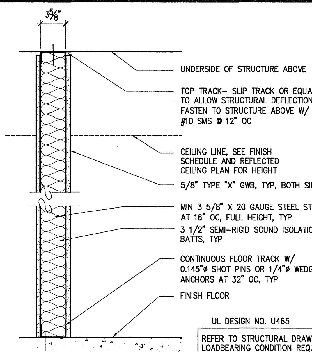
D 3 5/8" ONE-HOUR RATED PARTITION WALL SCALE: 1 1/2"=1'-0"
