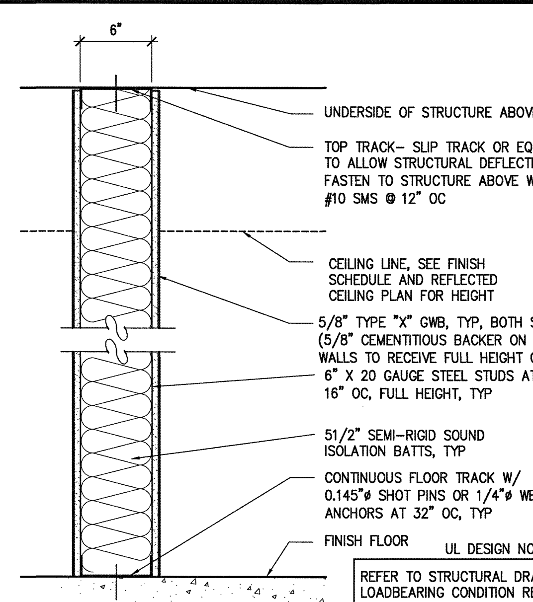
C 6" PARTITION WALL SCALE: 1 1/2"=1'-0"
