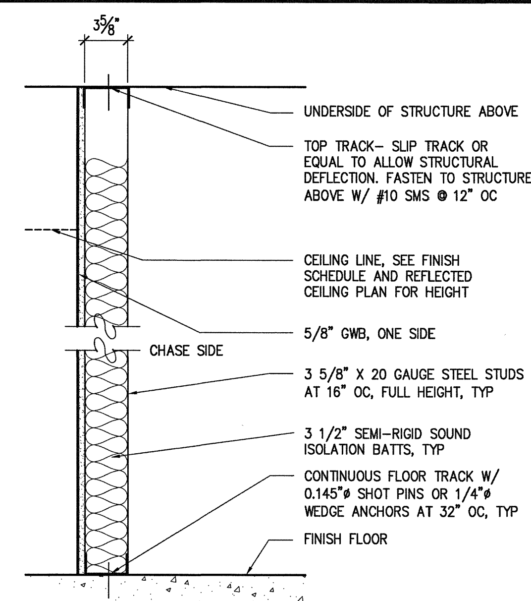
B 3 5/8" CHASE WALL SCALE: 1 1/2"=1'-0"
