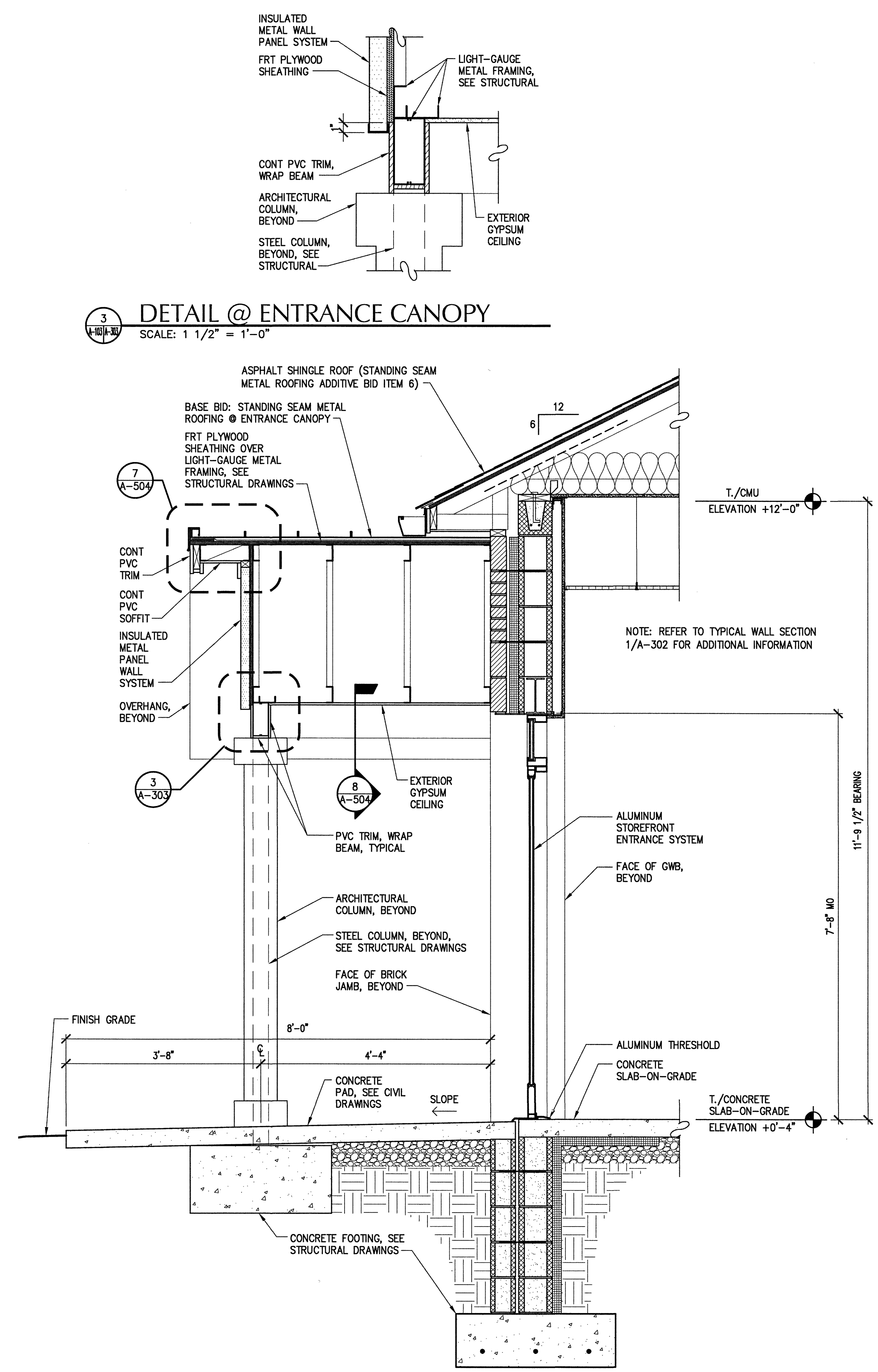
2 SECTION @ ENTRANCE CANOPY SCALE: 3/4" = 1'-0"
