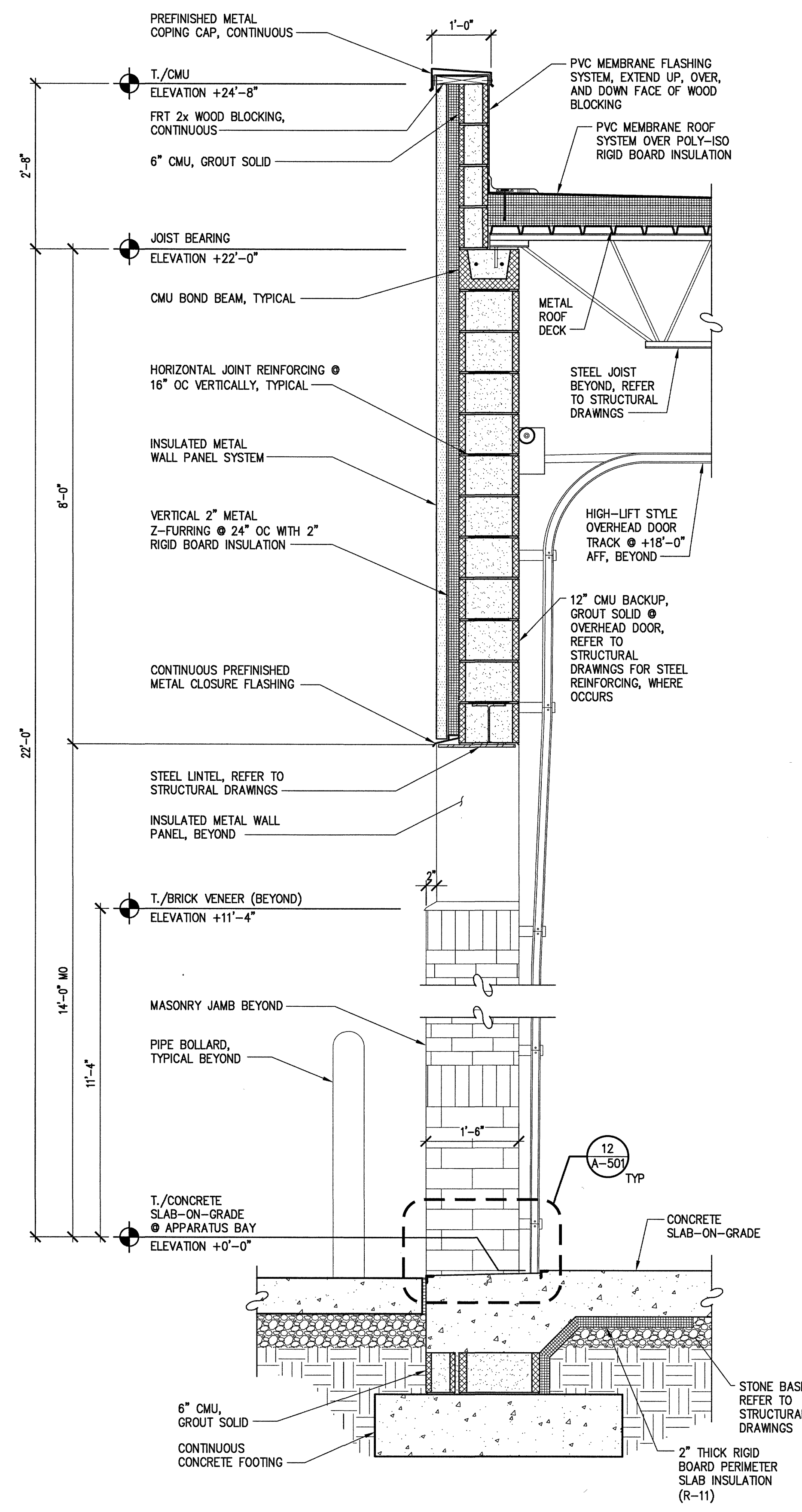
1 WALL SECTION @ APPARATUS BAY DOOR SCALE: 3/4" = 1'-0"
