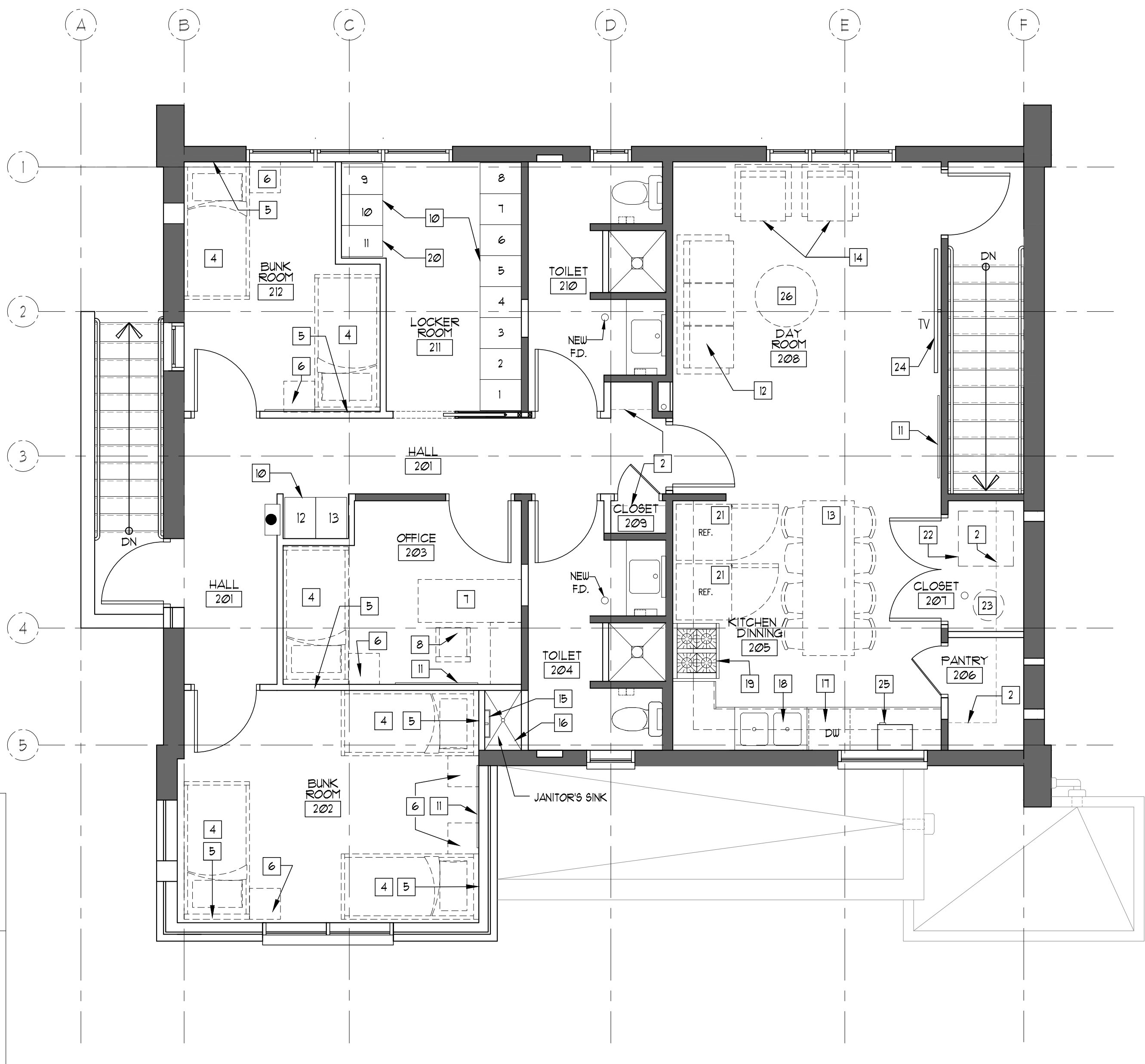
2 2nd FLOOR FURNITURE AND EQUIPMENT PLAN ID.2 SCALE: 1/4"=1'-0"
